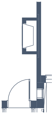
OPTIONAL EXTENDED GAS FIREPLACE
