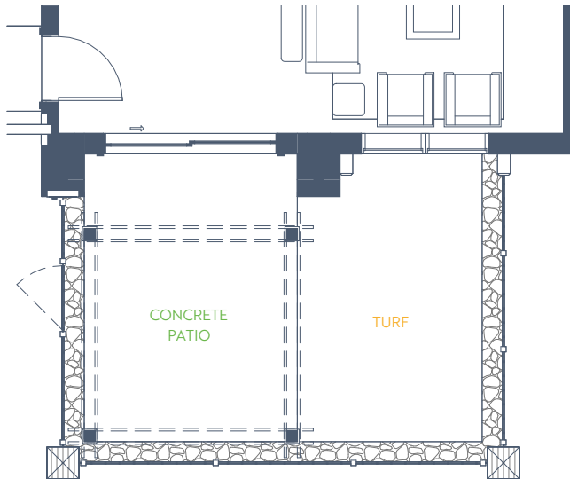
CONCRETE PATIO w/ OPT TURF
