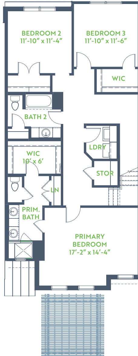
2 ND FLOOR 9' Ceiling
