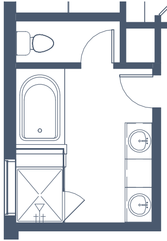
OPTIONAL PRIMARY BATH NO STEP SHOWER
